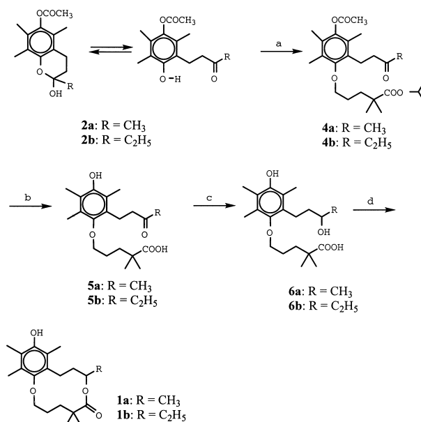
Scheme 1. Synthesis of 14-hydroxy-2,8-dioxabicyclo[10.4.0]hexadec-12,14,16-trien-7-ones 1a–b . (a) 1. NaH/DMSO, benzene; 2. 2,2-dimethyl-5-bromopentanoic acid, isopropyl ester ( 3 ). (b) KOH/EtOH. (c) NaBH 4 /MeOH. (d) 2,2'-dipyridyl disulfide, PPh 3 , CH 3 CN, AgClO 4 .
